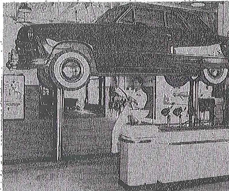
The Roswell Motor Company has in the new service department the latest Lincoln lubricating equipment to service your vehicles. Here LaWayne Carruth services a new Ford with the equipment. Note the Weaver twin post lift which gives easy access to any part on the underside.
