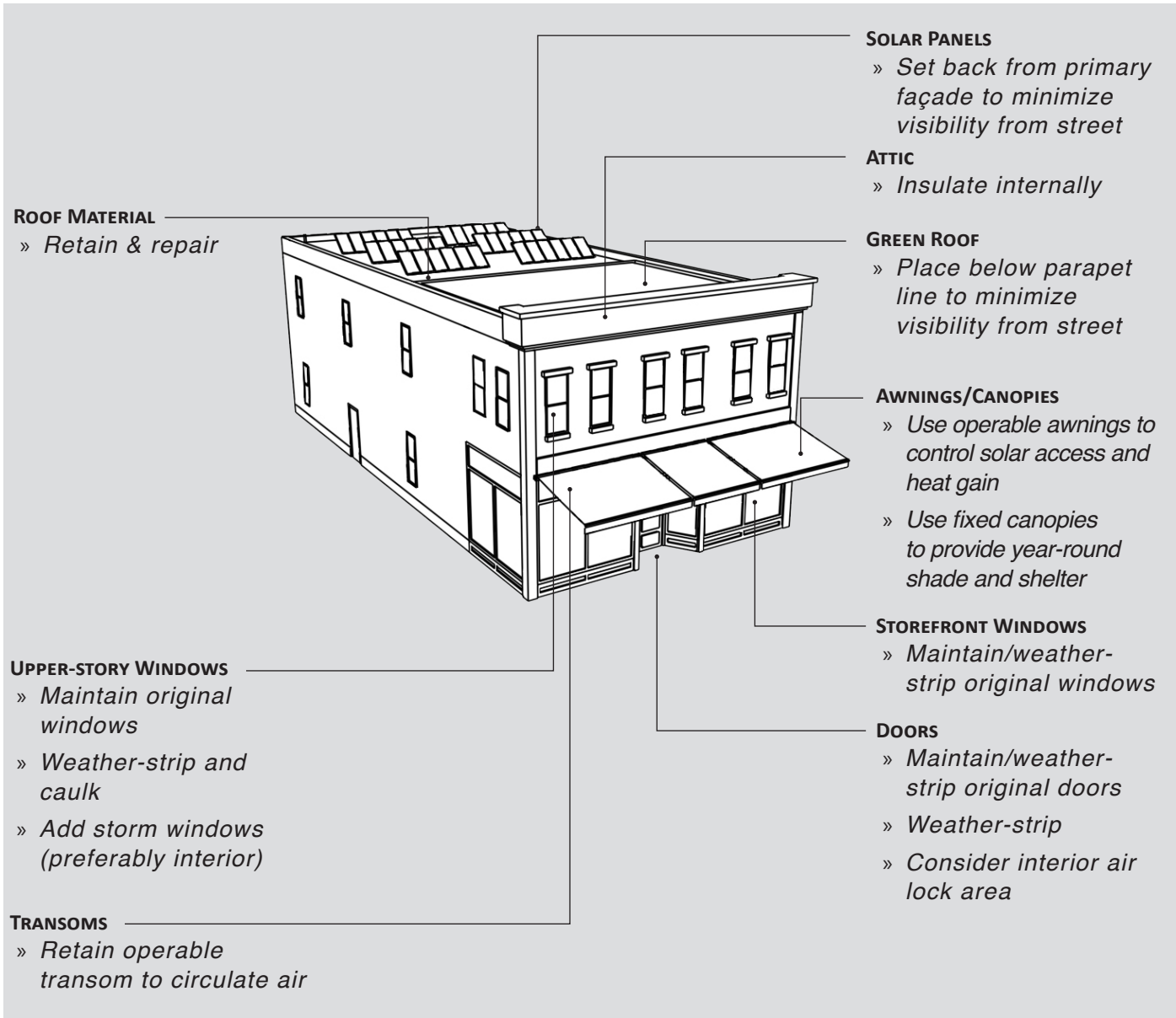
Figure 35: Commercial Building Energy Efficiency Diagram
