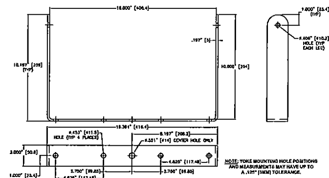
MOUNTING YOKE DETAIL
